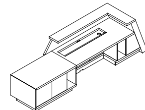
TJ58.3780 W3780*D950*H1110
