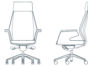
CGH80-1STG (780W*650D*H1180)
